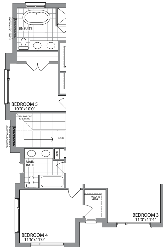
OPT. SECOND FLOOR W/5 BEDROOMS ELEVATION 3C
