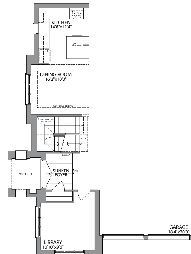
GROUND FLOOR ELEVATION 4C
