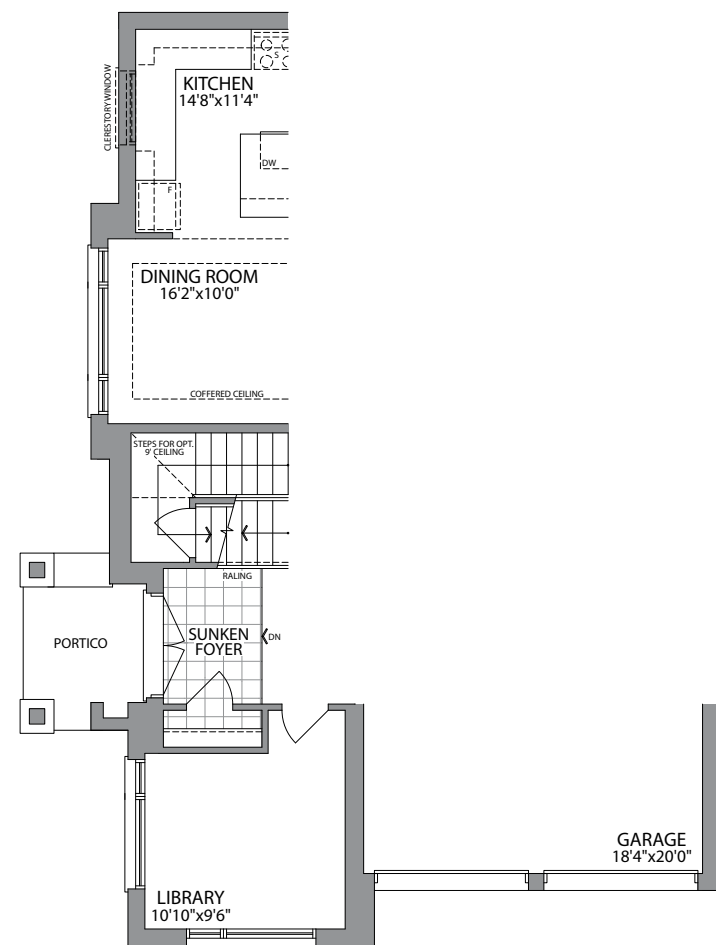
GROUND FLOOR ELEVATION 3C
