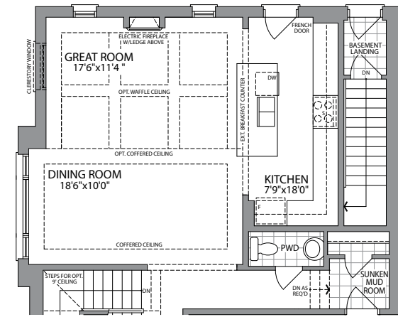
OPT. GROUND FLOOR W/OPT. BASEMENT ACCESS ELEVATION 3C
