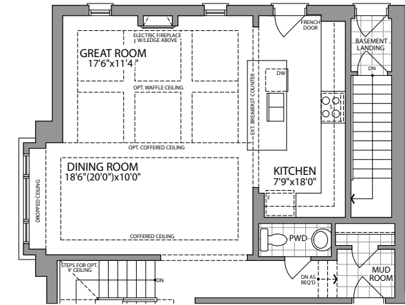
OPT. GROUND FLOOR W/OPT. BASEMENT ACCESS ELEVATION 2C
