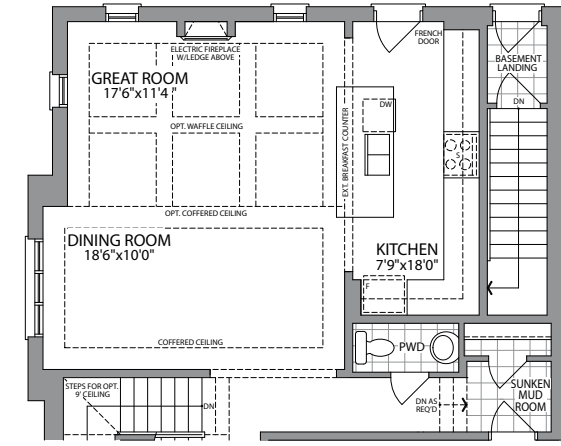
OPT. GROUND FLOOR W/OPT. BASEMENT ACCESS ELEVATION 4C
