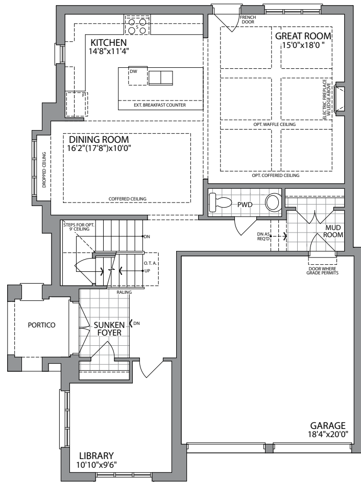
GROUND FLOOR ELEVATION 1C
