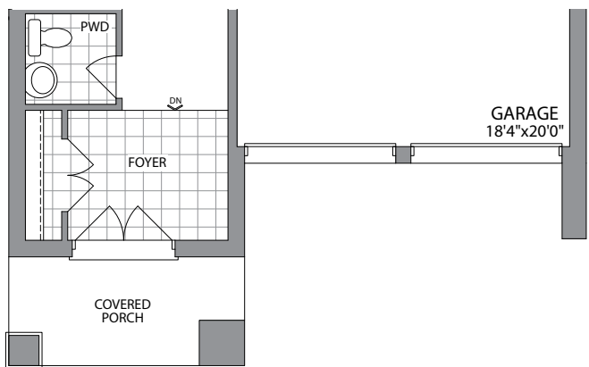
GROUND FLOOR ELEVATION 2
