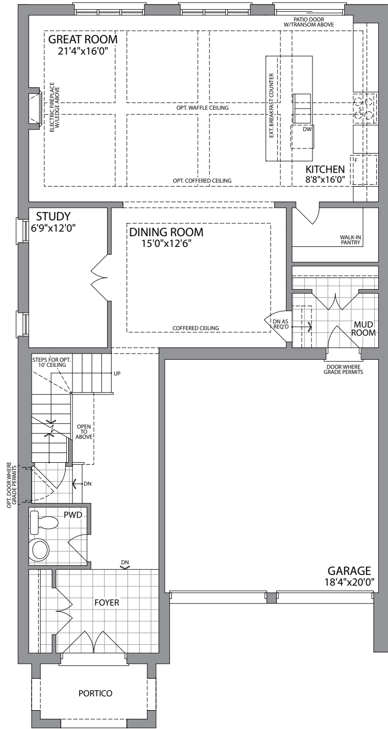
GROUND FLOOR ELEVATION 1 & 4
