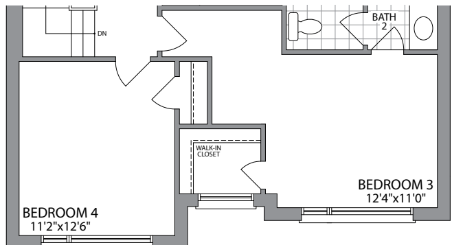
SECOND FLOOR ELEVATION 3
