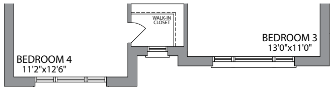
SECOND FLOOR ELEVATION 4
