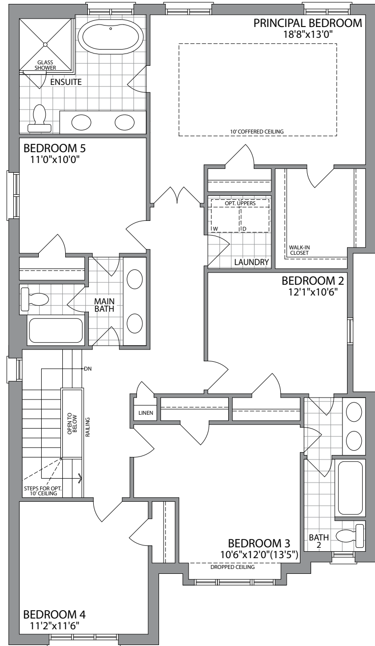
SECOND FLOOR ELEVATION 1
