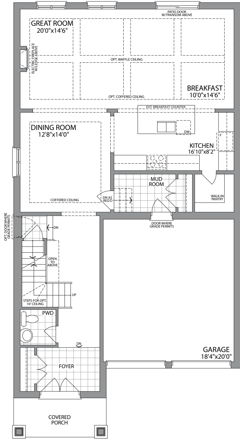
GROUND FLOOR ELEVATION 1
