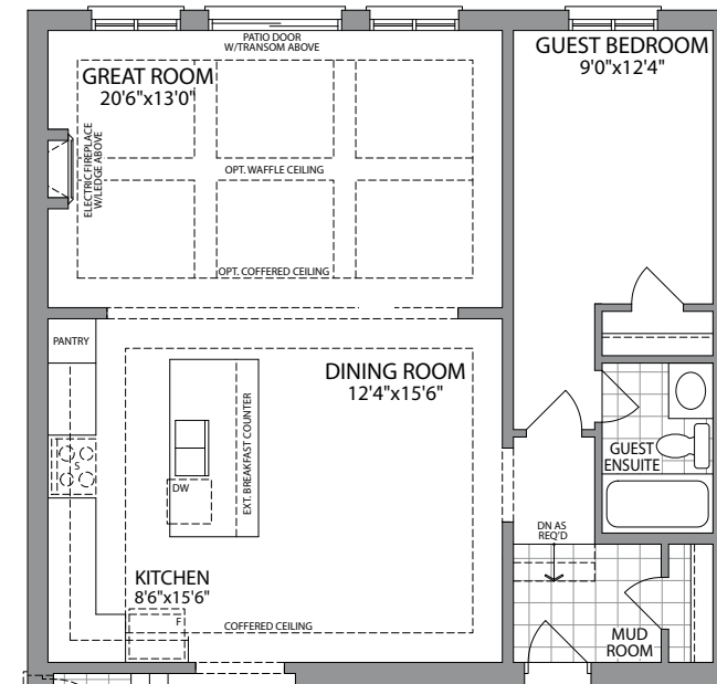
OPT. GROUND FLOOR W/GUEST BEDROOM ELEVATION 1, 2, 3 & 4
