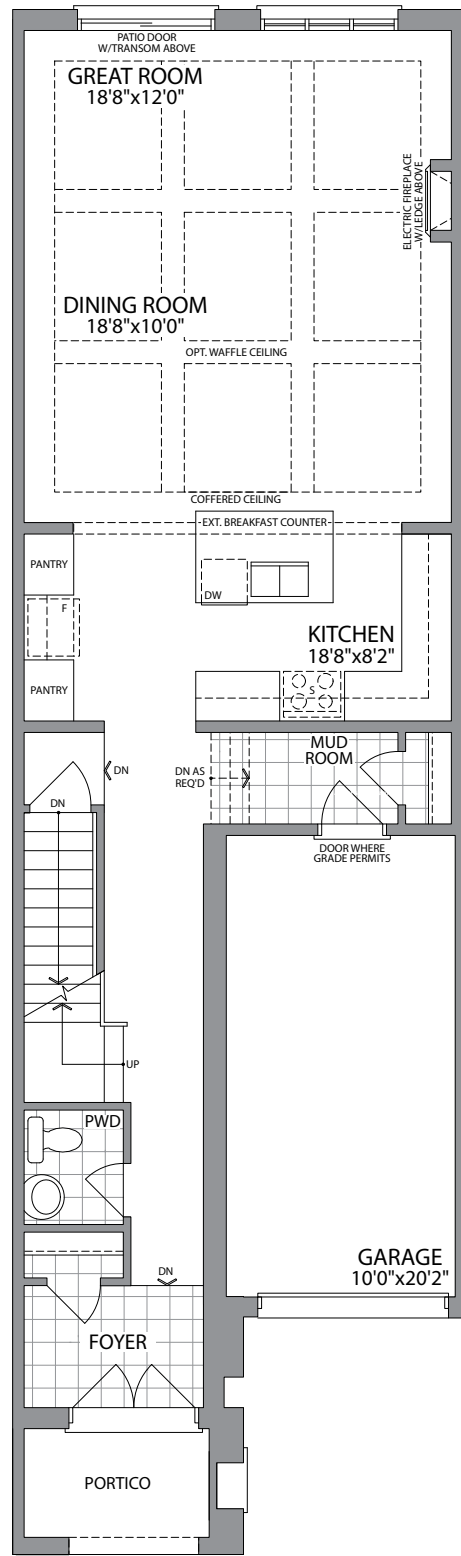
GROUND FLOOR ELEVATION 1
