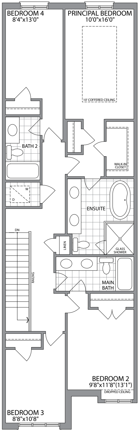
SECOND FLOOR ELEVATION 1
