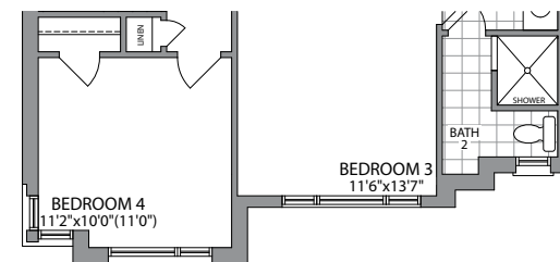
SECOND FLOOR ELEVATION 2
