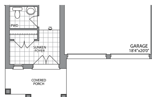
GROUND FLOOR ELEVATION 4
