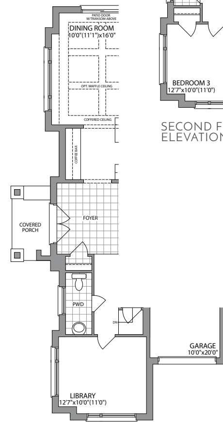
GROUND FLOOR ELEVATION 3C
