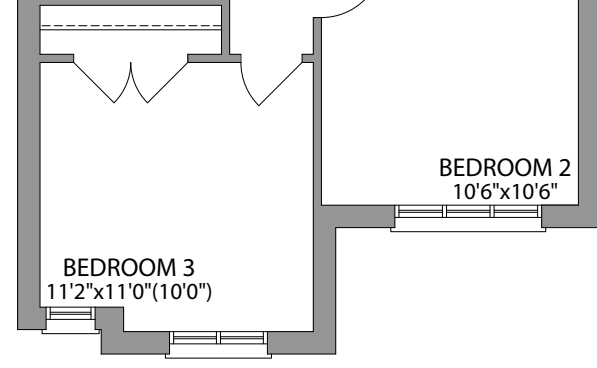
SECOND FLOOR ELEVATION 4
