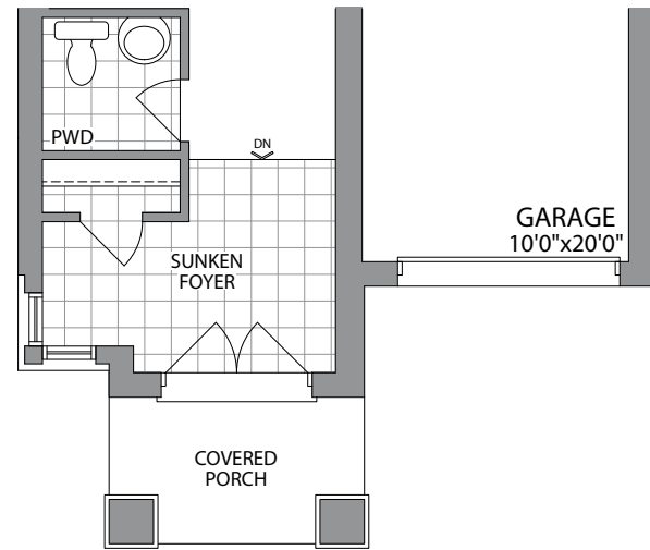
GROUND FLOOR ELEVATION 2
