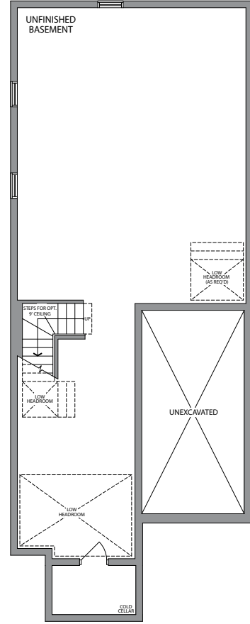
BASEMENT ELEVATION 1
