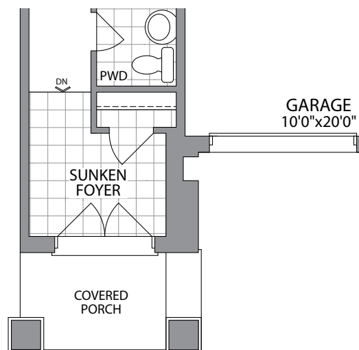
GROUND FLOOR ELEVATION 2
