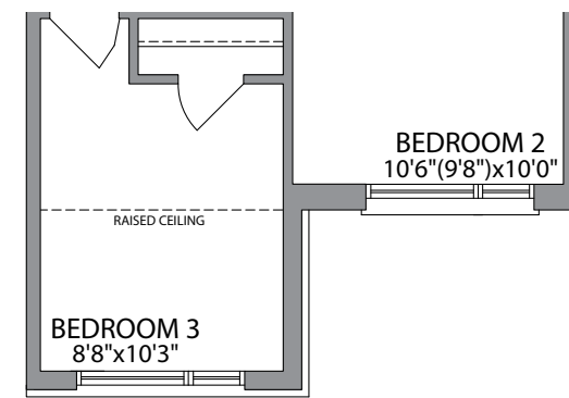
OPT. SECOND FLOOR W/4 BEDROOMS ELEVATION 2
