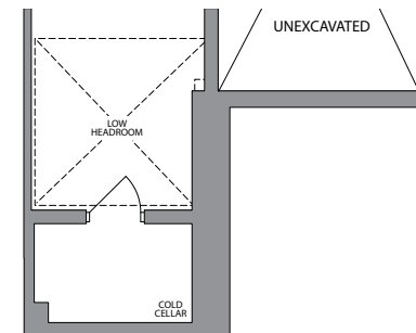
BASEMENT ELEVATION 2
