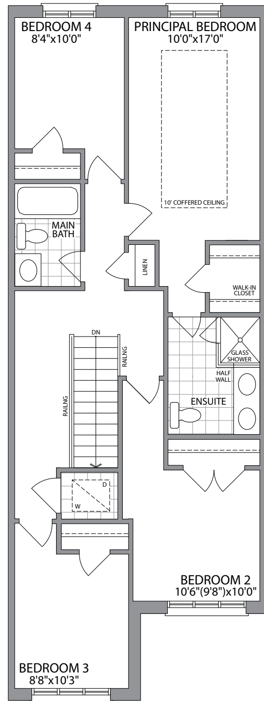
OPT. SECOND FLOOR W/4 BEDROOMS ELEVATION 1
