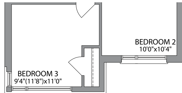
SECOND FLOOR ELEVATION 2
