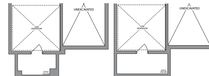
BASEMENT ELEVATION 2
