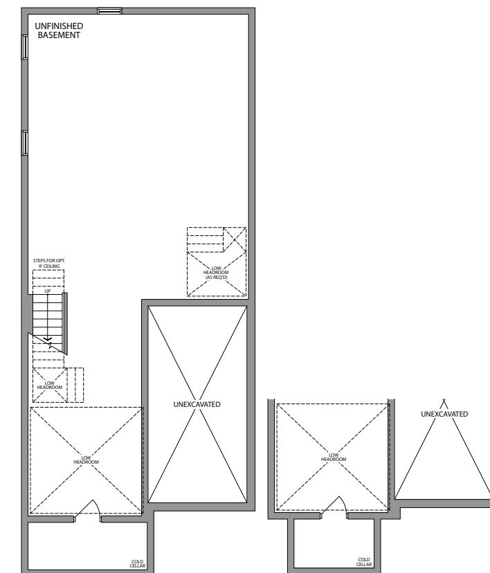
BASEMENT ELEVATION 3
