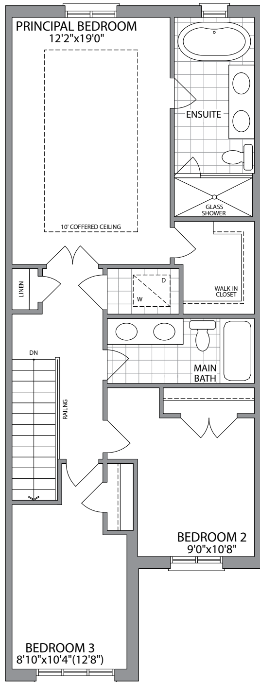
SECOND FLOOR ELEVATION 1
