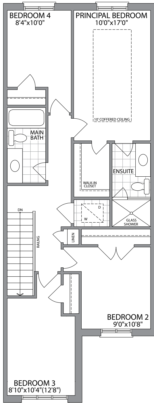
OPT. SECOND FLOOR W/4 BEDROOMS ELEVATION 1 (ELEVATION 3 SIMILAR)
