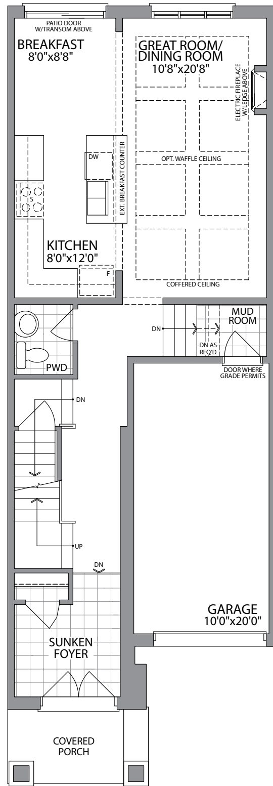
GROUND FLOOR ELEVATION 1
