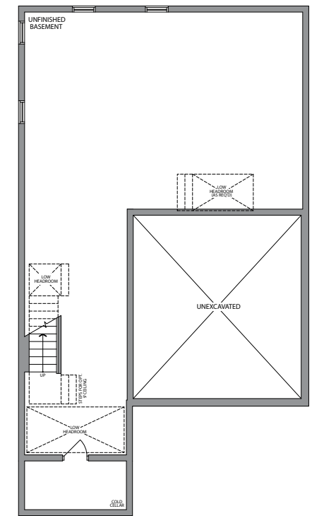
BASEMENT ELEVATION 1
