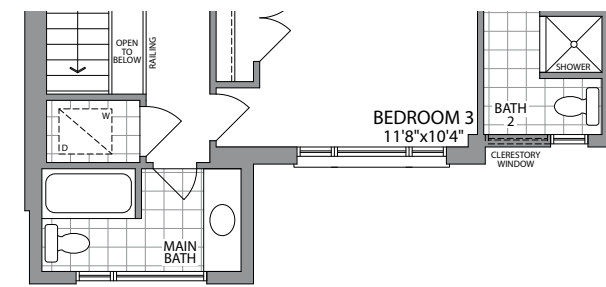
OPT. SECOND FLOOR W/5 BEDROOMS ELEVATION 2
