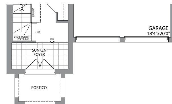
GROUND FLOOR ELEVATION 3
