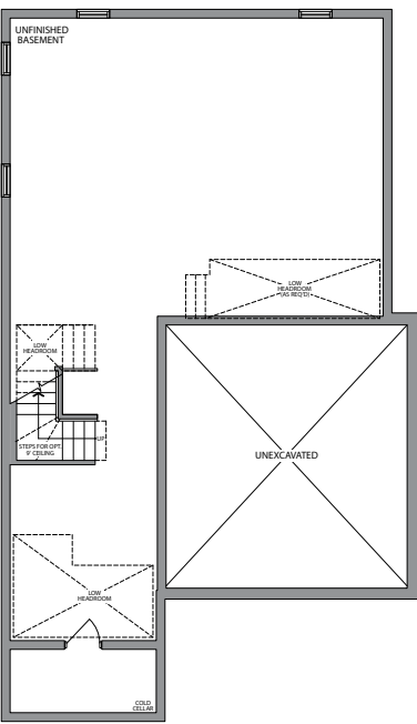
BASEMENT ELEVATION 1
