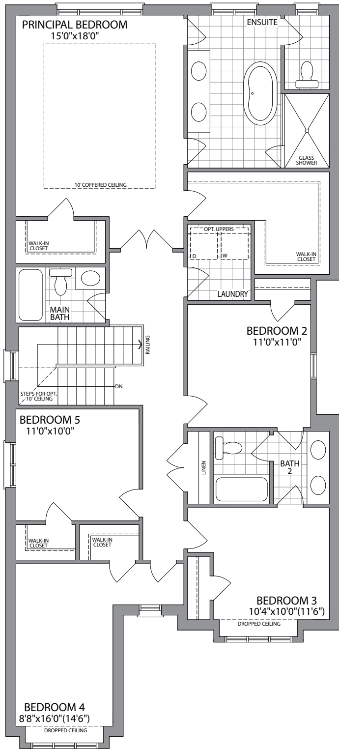
SECOND FLOOR ELEVATION 1
