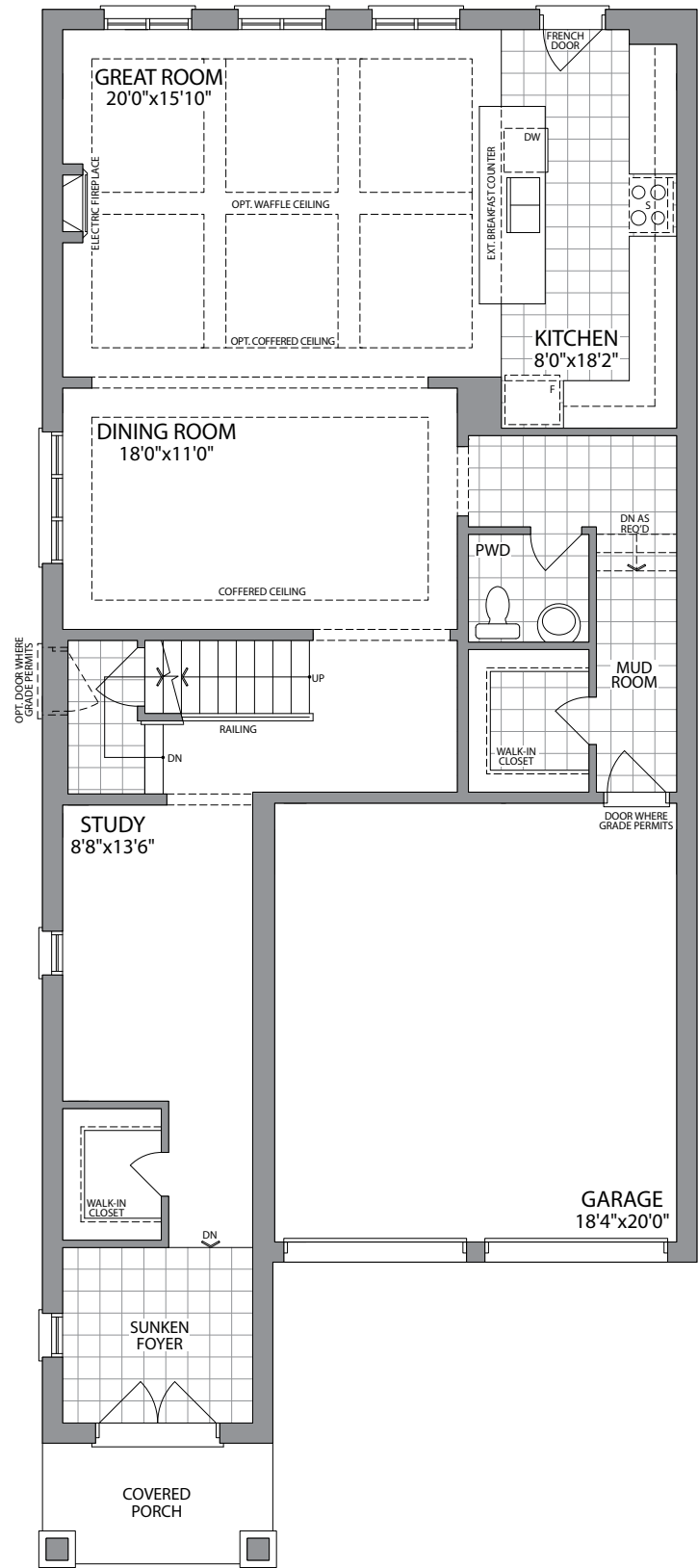
GROUND FLOOR ELEVATION 1 & 2
