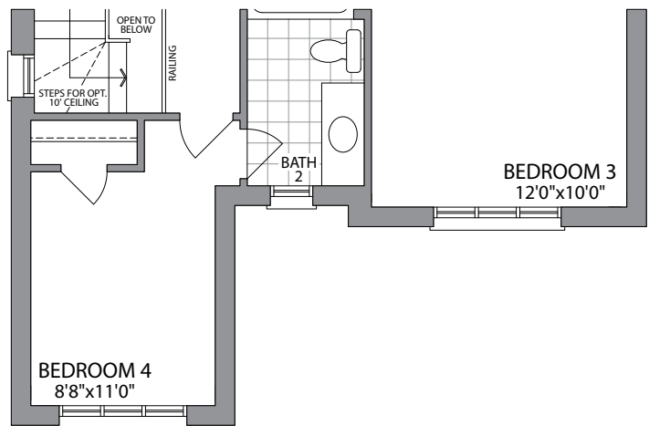
OPT. SECOND FLOOR W/5 BEDROOMS ELEVATION 2
