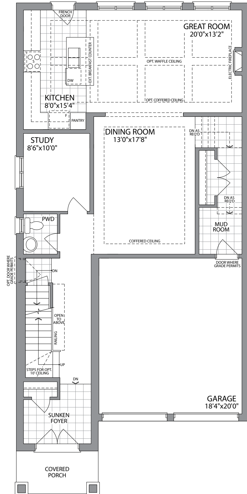
GROUND FLOOR ELEVATION 1 & 2
