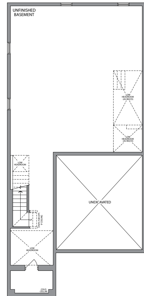
BASEMENT ELEVATION 1 & 2
