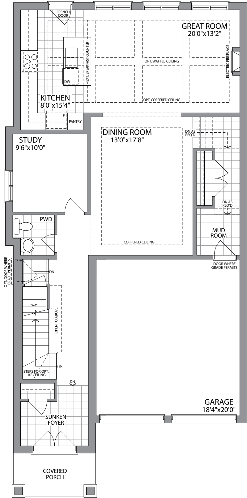
GROUND FLOOR ELEVATION 1C
