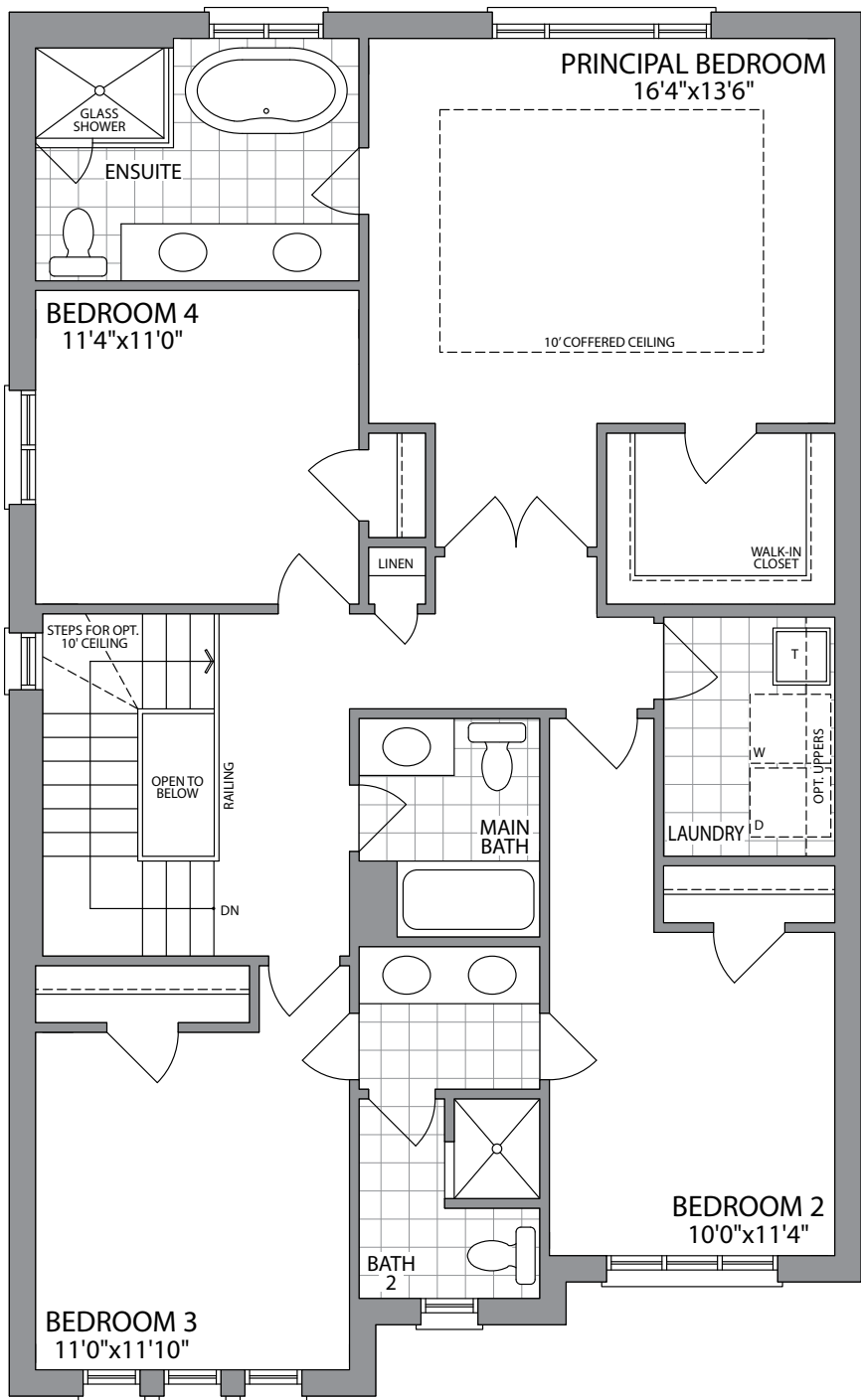
SECOND FLOOR ELEVATION 1
