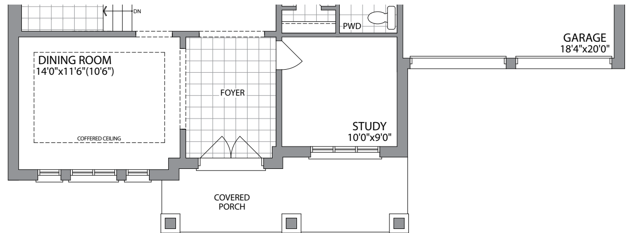
GROUND FLOOR ELEVATION 2
