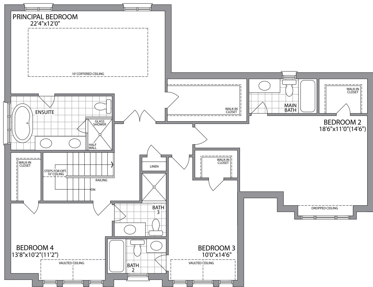
SECOND FLOOR ELEVATION 1
