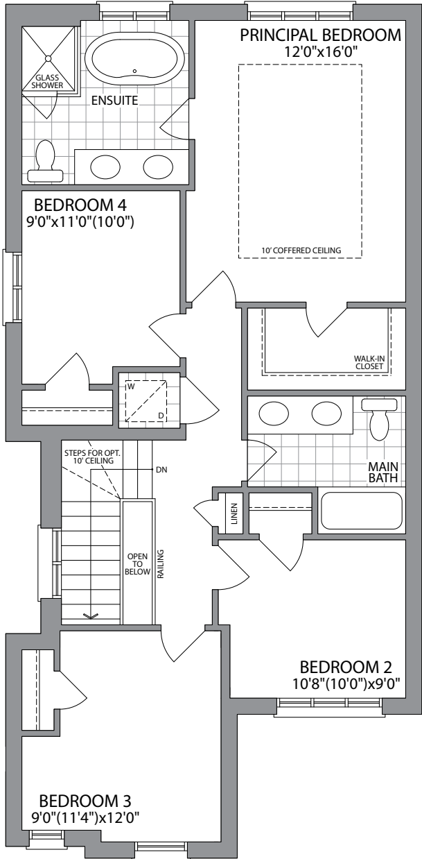
OPT. SECOND FLOOR W/4 BEDROOMS ELEVATION 1
