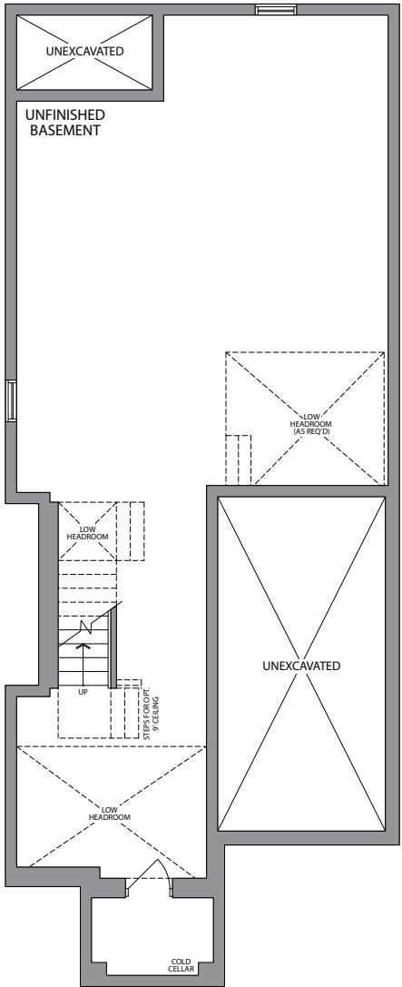
BASEMENT ELEVATION 1
